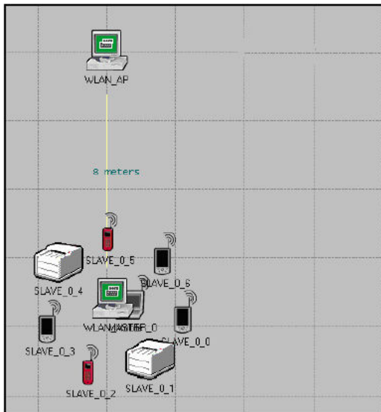
Figure 2. Scenario 2 – WLAN and PICONET with 7 slaves
