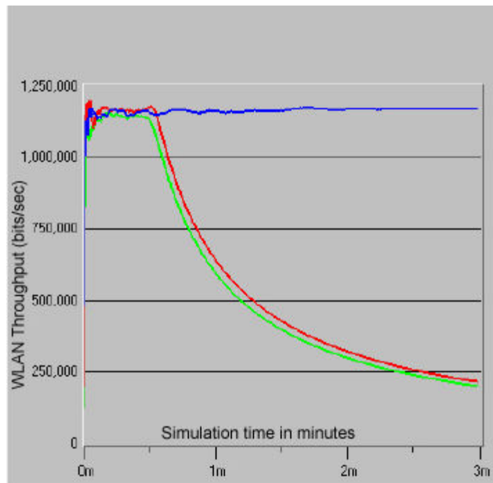
Figure 5. WLAN throughput (bits/sec) comparison between the scenarios
