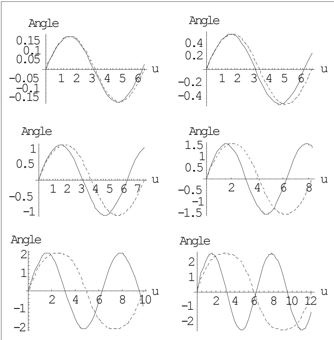
Fig.3. Swing angle vs. time, for \alpha \approx 10^\circ, 30^\circ, 60^\circ, 90^\circ, 120^\circ, and 150^\circ . Exact values are for \alpha \approx 10^\circ, 30.32^\circ, 63^\circ, 88.420^\circ, 121.3^\circ, and 147^\circ . Solid lines (approximate solution); dashed lines (exact solution)
