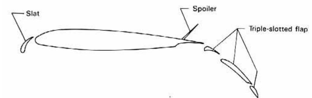
Figure 5 Flaps – an example of inventive principle #7 nesting
