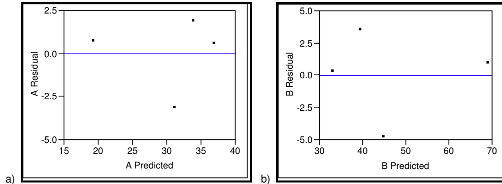
Figure 7. Residual versus predicted plots for the grades A (a) and B (b).
