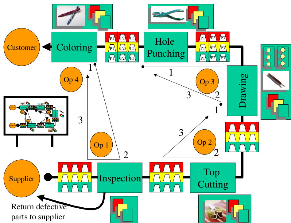
Figure 2: Production layout for lean manufacturing
