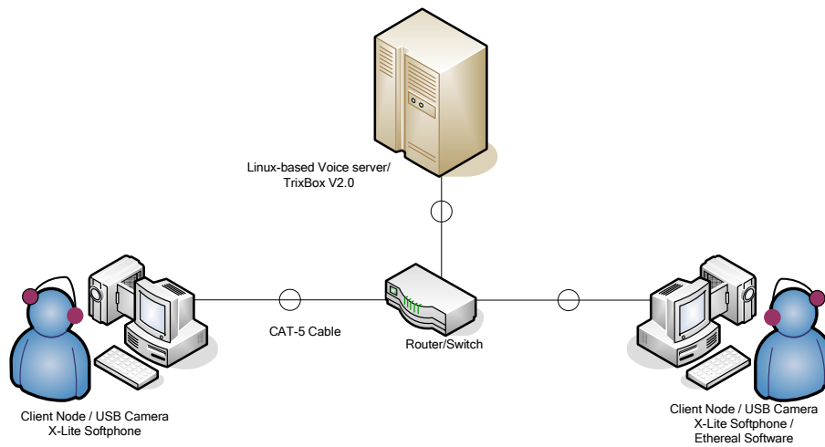
Figure 1: Network configuration of the VoIP system.
