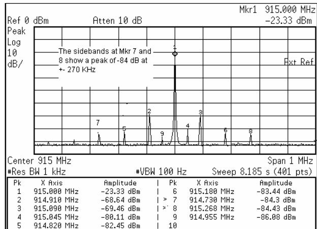
Figure 7, Reflected 915 MHz signal, using fixture FL1 with four lamps ON, (Modulated sidebands clearly shown spaced at 45 KHZ bands)
