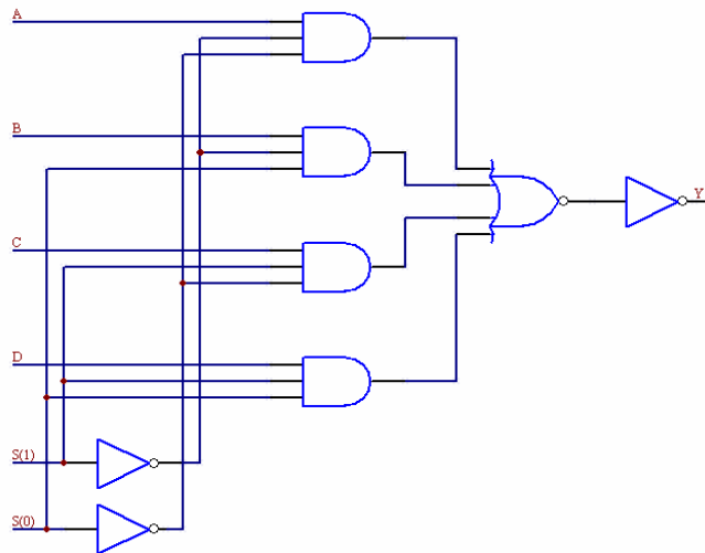
Fig. 7. Synthesized MUX Circuit from Code 1 and 2
