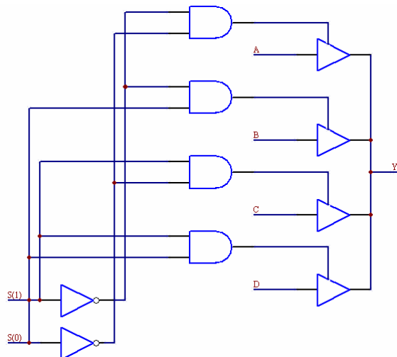
Fig. 8. Synthesized MUX Circuits from Code 3
